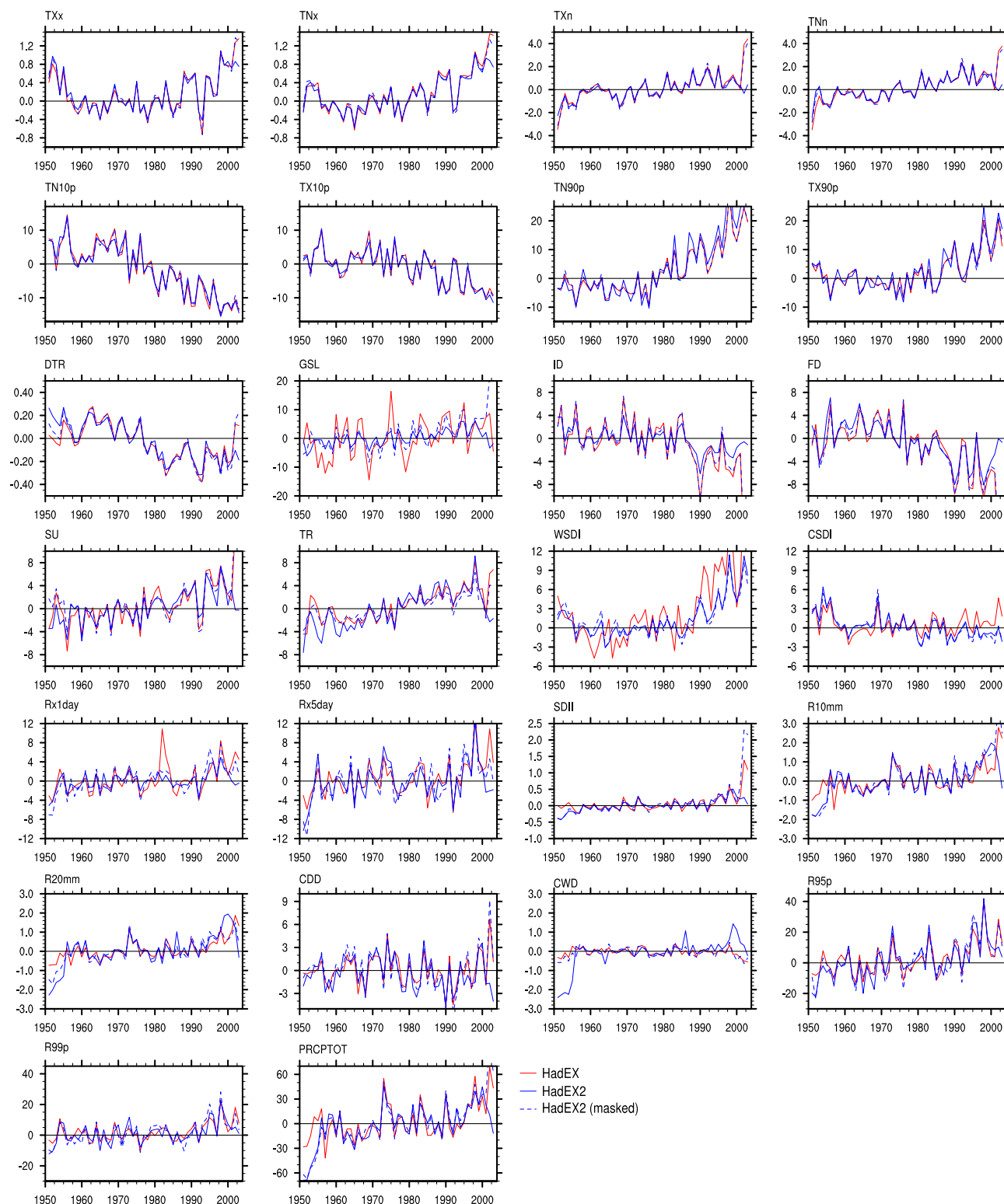
Figure A1. Global average time series of annual index values (anomalies relative to 1961–1990 mean values) for 26 of the Expert Team on Climate Change Detection and Indices (ETCCDI) core indices for HadEX2 (blue lines) in comparison to HadEX (red lines; A2006) over the 1951–2003 period (for which HadEX had data). For the calculation of global averages, only grid boxes with at least 90% of \ coverage are used, i.e., 48 years during 1951–2003. HadEX2 is also masked to grid boxes where HadEX had data (blue dashed lines) to show that most of the differences can be attributed to different spatial coverage. Units as indicated in Table 1.
